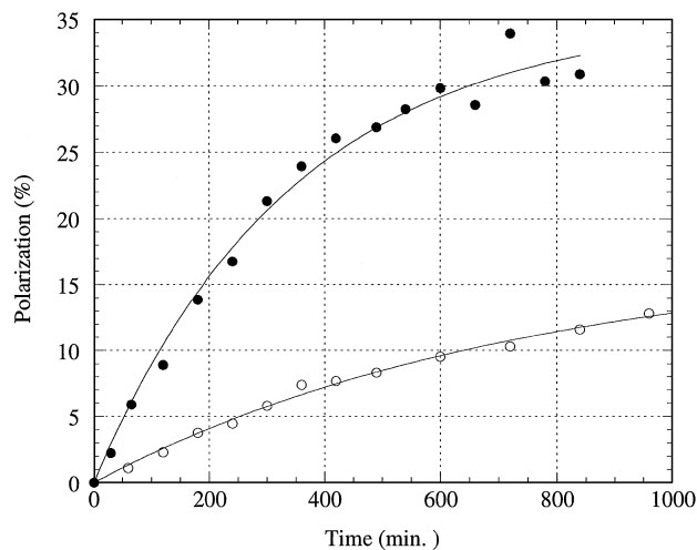
FIG. 2. Buildup of the proton polarization at 0.3 T and 77 K. The data shown as closed circles were obtained with the pulsed dye laser at 600 nm and 350 mW for a single crystal of naphthalene doped with about 0.001 mol% of pentacene. The buildup time of 343 min and the extrapolated maximum proton polarization P_{p0} of 35.3% were obtained by fitting the data to the simple exponential in Eq. (3). The data shown as open circles were obtained with the pulsed N_2 laser at 337 nm and 150 mW for a single crystal of naphthalene doped with about 0.01 mol% of pentacene.
