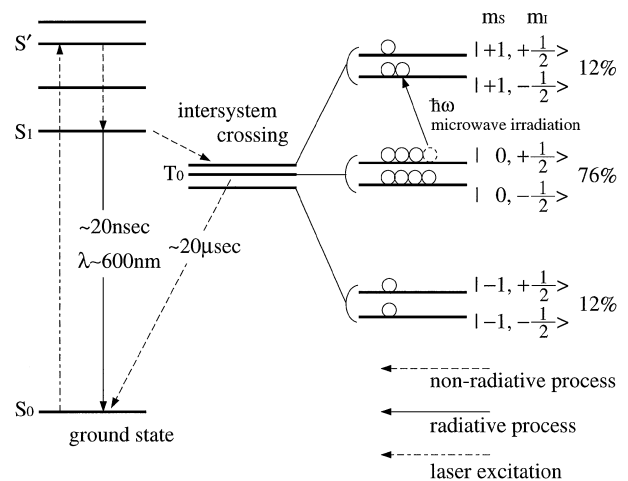
FIG. 1. Energy levels of pentacene: The values on the right side represent the populations of sublevels in the lowest triplet state T_0 . The singlet states S' and S_1 are optically excited states.
