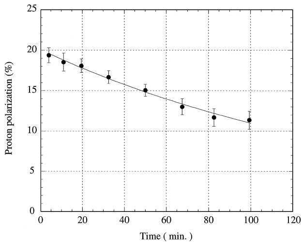
FIG. 3. Decay of the proton polarization in the naphthalene crystal without laser beam at 0.0007 T and 77 K measured by the neutron transmission method. The polarization and the relaxation time of proton were obtained to be 20.0\% \pm 3.6\% and 166 \pm 22 min, respectively.
