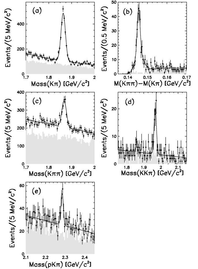
FIG. 1. Invariant mass distributions of charm-hadron candidates in 107 pb ^{-1} of inclusive electron data. (a) K\pi invariant mass distribution for \bar{D}^0 candidates. (b) Mass difference distribution, \Delta M = M(K\pi\pi) - M(K\pi) , for D^{*-} candidates. (c) K\pi\pi invariant mass distribution for D^- candidates. (d) KK\pi invariant mass distribution for D_s^- candidates. (e) pK\pi invariant mass distribution for \Lambda_c^- candidates. The shaded histograms represent the combinations with the wrong electron-hadron charge correlation. The shaded area in (a) has been scaled by 0.5 for display purposes.
