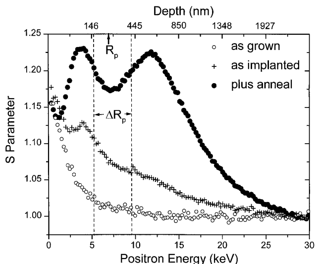
FIG. 1. S parameters as a function of positron energy for MgO samples that are as-grown (open circles), Au ion-implanted (crosses), and annealed at \sim 1200^\circ\text{C} for 90 min in Ar + 5%O 2 after implantation (solid circles). The implant parameters for high-energy implantation at 1.1 MeV with a dose of 6 \times 10^{16} ions/cm 2 . The S parameter of bulk MgO is normalized to be one.
