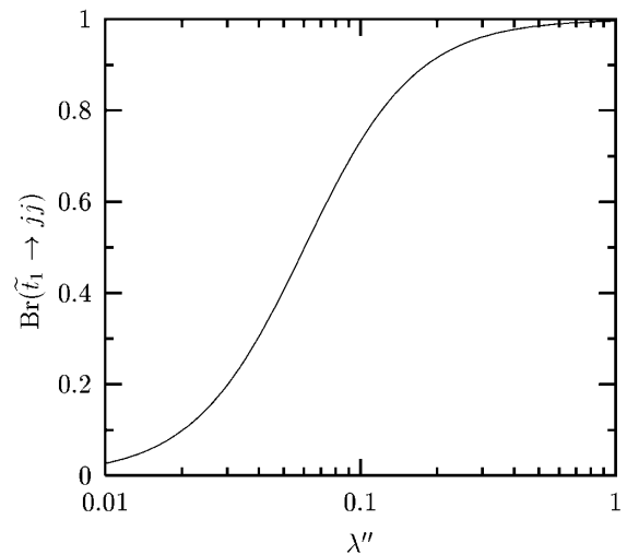
FIG. 2. Branching ratio for the top squark to decay into two jets via the R -parity-violating coupling \lambda'' as a function of the coupling.
