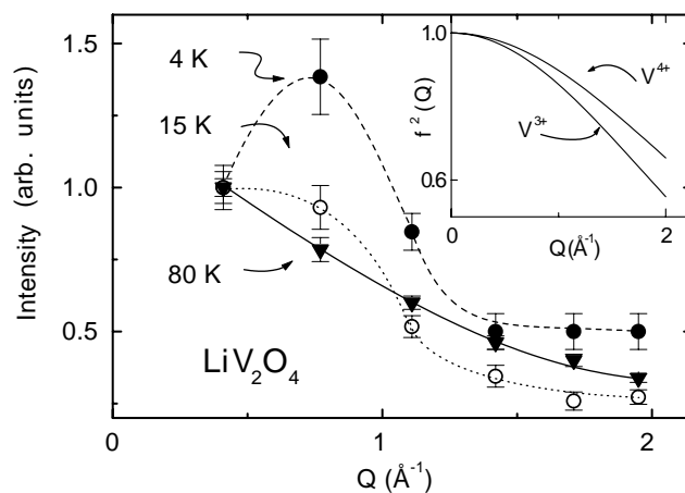
FIG. 2. Q dependence of the energy-integrated intensity of the quasielastic scattering of \text{LiV}_2\text{O}_4 at 4, 15, and 80 K, respectively. For comparison, the inset shows the Q dependence according to the square of the neutron magnetic form factor of the two vanadium configurations possible in \text{LiV}_2\text{O}_4 . The maximum around Q = 0.76 \text{ \AA}^{-1} at 4 K corresponds to the reciprocal lattice spacing a^* . Dashed or dotted lines are guides to the eye.
