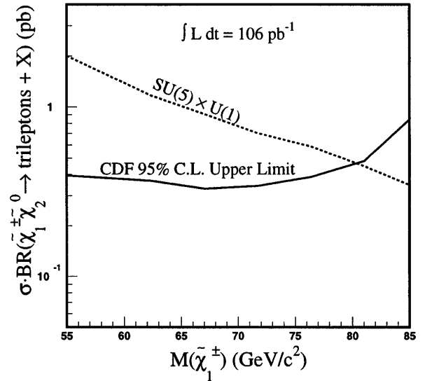
FIG. 3. \sigma \text{BR}(\tilde{\chi}_1^\pm \tilde{\chi}_2^0 \rightarrow 3\ell + X) versus \tilde{\chi}_1^\pm mass for the SU(5) \times U(1) model [19]. This sets a mass limit of 80.5 \text{ GeV}/c^2 . In this model, the \tilde{\ell}_R is lighter than the \tilde{\chi}_2^0 , resulting in two body decays of the \tilde{\chi}_2^0 . Note that the acceptance for events from this model decreases at large \tilde{\chi}_1^\pm mass. In this region, the LSP mass approaches that of the \tilde{\ell} , resulting in soft final state leptons which are difficult to detect.
