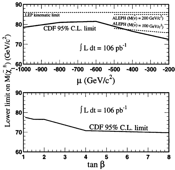
FIG. 2. The experimental limit on M_{\tilde{\chi}_1^\pm} as a function of \mu for \tan \beta = 2 and M_{\tilde{q}} = M_{\tilde{g}} (upper) and as a function of \tan \beta for \mu = -400 \text{ GeV}/c^2 and M_{\tilde{q}} = M_{\tilde{g}} (lower). The ALEPH limits shown [17] are from a search for all possible final states. In this analysis M_{\tilde{\nu}} \approx 100 \text{ GeV}/c^2 . Minimal SUGRA models favor the region of small |\mu| values.
