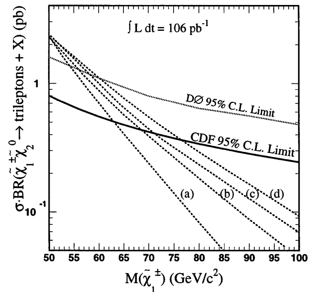
FIG. 1. \sigma \text{BR}(\tilde{\chi}_1^\pm \tilde{\chi}_2^0 \rightarrow 3\ell + X) versus \tilde{\chi}_1^\pm mass for representative points in the MSSM parameter space, namely \mu = -400 \text{ GeV}/c^2 , \tan\beta = 2 , and (a) M_{\tilde{q}}/M_{\tilde{g}} = 2.0 ; (b) M_{\tilde{q}}/M_{\tilde{g}} = 1.5 , (c) M_{\tilde{q}}/M_{\tilde{g}} = 1.2 , and (d) M_{\tilde{q}}/M_{\tilde{g}} = 1.0 . BR is the summed branching ratio into the four trilepton modes ( e^+e^-e , e^+e^-\mu , e\mu^+\mu^- , and \mu^+\mu^-\mu ). The solid line is the 95% confidence level upper limit based on an observation of zero events. We set a mass limit of 77.0 \text{ GeV}/c^2 when M_{\tilde{q}} = M_{\tilde{g}} . All MSSM points in this plot yield three body decays of the \tilde{\chi}_1^\pm and \tilde{\chi}_2^0 . The D0 limit [15] is for a single trilepton mode which we scale up by 4 to match our notation.
