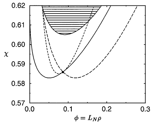
FIG. 2. A cut through the phase behavior in Fig. 1 by the physical ( \phi = L_N \rho, \chi ) plane showing the cloud curve (solid line), shadow curve (long-dashed line), spinodal curve (dashed line), and the critical point. Also shown for comparison is the two phase region for the monodisperse Flory-Huggins theory with the same mean chain length, L = 100 .
