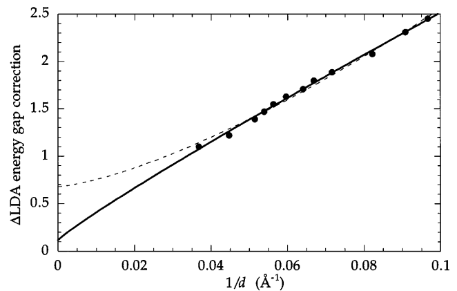
FIG. 1. The band-gap correction from Ref. [1] plotted against the inverse cluster diameter. The best fit (solid curve) correctly tends to a value consistent with zero.
