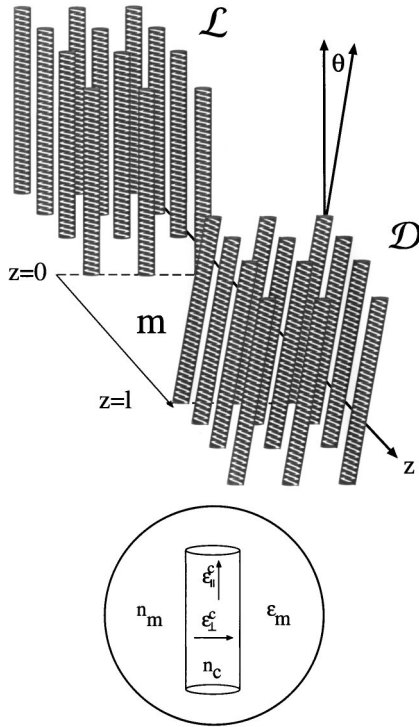
FIG. 1. Array-interaction geometry. Region \mathcal{L} is confined to z < 0 , region \mathcal{D} to z > l ; isotropic region m is the slab in between. The cylindrical array in \mathcal{D} is rotated about the z axis by an angle \theta with respect to \mathcal{L} . Not only the dielectric constants of the composite media \mathcal{D} and \mathcal{L} but also the dielectric constants of the cylindrical rods (bottom) themselves are anisotropic; \epsilon_{\parallel}^c , \epsilon_{\perp}^c , n_c refer to the cylinder material.
