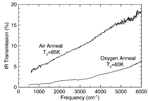
FIG. 1. IR transmission at T = 300 K of the same overdoped Bi2212 crystal before and after an anneal in air.
