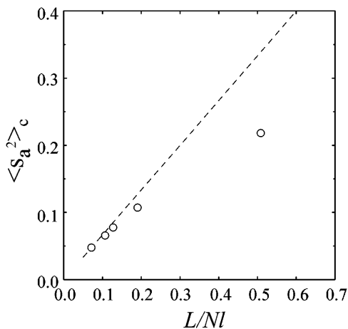
FIG. 5. Dependence of the second cumulant \langle s_a^2 \rangle_c upon sample dimensions.
