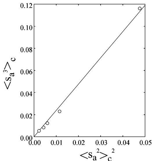
FIG. 3. Plot of \langle s_a^3 \rangle_c versus \langle s_a^2 \rangle_c^2 . The solid line represents a least square linear fit to the data.
