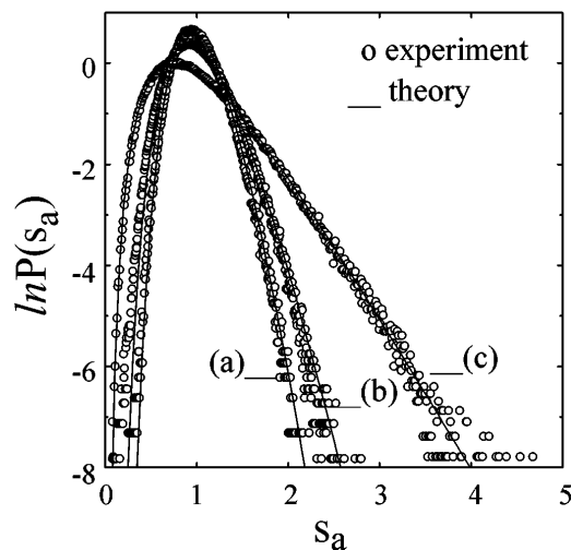
FIG. 2. Semilogarithmic plot of the transmission distributions for the same samples as in Fig. 1.
