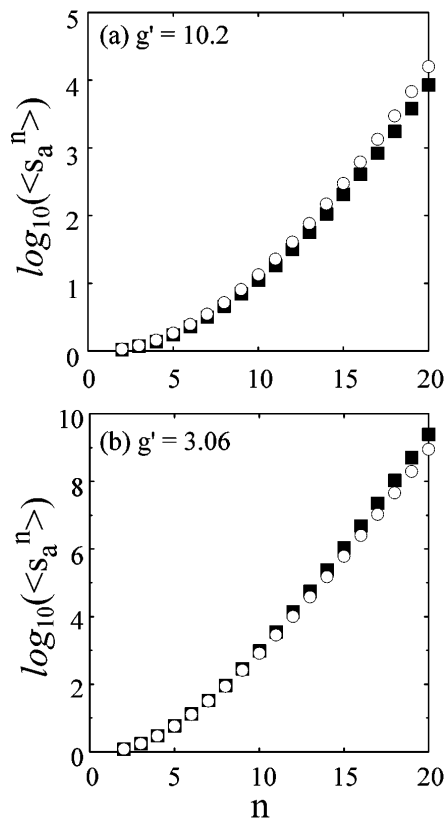
FIG. 4. Comparison of the calculated (circles) and measured (squares) moments of the transmission distribution for samples with (a) g' = 10.2 and (b) g' = 3.06 .
