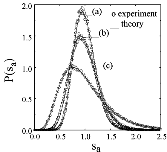
FIG. 1. Distribution function of the normalized transmission P(s_a) for three samples with dimensions (a) d = 7.5 cm, L = 66.7 cm, (b) d = 5.0 cm, L = 50.0 cm, and (c) d = 5.0 cm, L = 200 cm.
