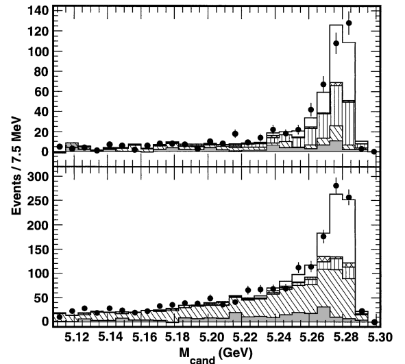
FIG. 1. M_{\text{cand}} distributions for the D^0l^- \bar{\nu} (top) and D^+l^- \bar{\nu} (bottom) modes. The points are the data, the shaded component is the continuum and fake lepton background, the diagonal hatch is the combinatoric background, the vertical hatch is the \bar{B} \rightarrow D^*l\bar{\nu} feeddown, and the crosshatch is the \bar{B} \rightarrow D^{**}l\bar{\nu} and other backgrounds. The unshaded area is the prediction of a Monte Carlo simulation of the signal, normalized to the measured decay rate.
