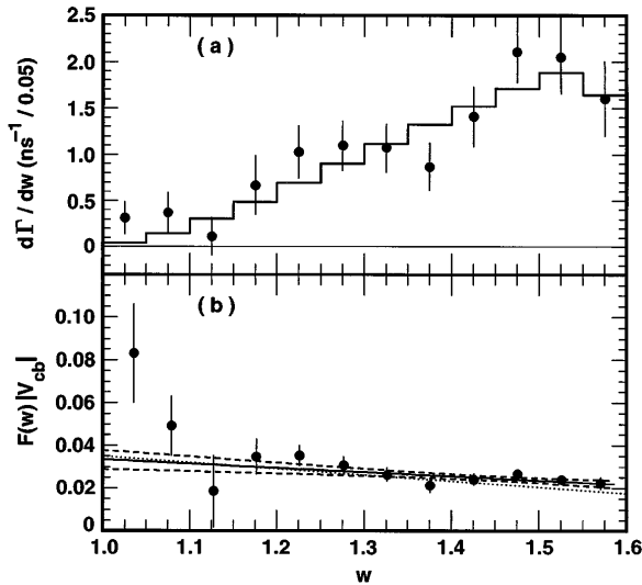
FIG. 2. (a) d\Gamma/dw distribution from the data (points), and the result of the \hat{c}_D = 0 fit to the distribution (histogram). (b) Measured values of \mathcal{F}_D(w) |V_{cb}| (points), the result of the fit (solid line) along with its statistical errors (dashed lines), and the function \mathcal{F}_{D^*}(w) |V_{cb}| obtained from an analysis of \bar{B} \rightarrow D^* l \bar{\nu} decays (dotted line).
