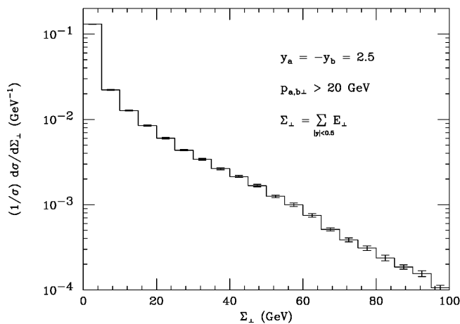
FIG. 4. The distribution of \Sigma_{\perp} as explained in the text.
