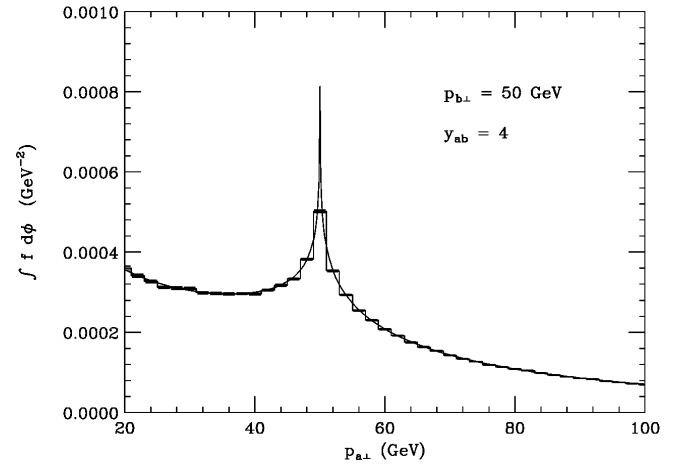
FIG. 3. Comparison of the Monte Carlo solution (histogram) with the standard solution to BFKL (solid).
