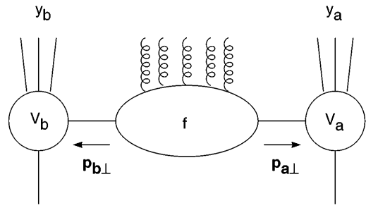
FIG. 1. A schematic picture of the cross section for producing particles at large rapidity separation.
