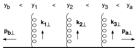
FIG. 2. The amplitude for three gluon emissions in the BFKL approximation.
