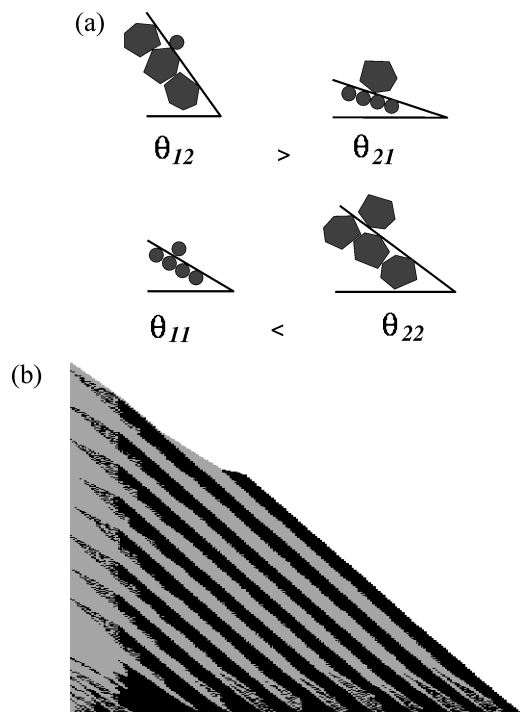
FIG. 1. (a) The slopes of repose s_{\alpha\beta} depend on the composition of grains at the surface of the pile and are chosen according to the four possible interactions between small and large grains. The slopes of repose satisfy s_{21} < s_{11} < s_{22} < s_{12} (see discussion in text). (b) The result obtained with the discrete model (for H_1 = 1 , H_2 = 2 , s_{21} = 2 , s_{11} = 6 , s_{22} = 7 , s_{12} = 10 , N_1 = 20 , and N_2 = 10 ).
