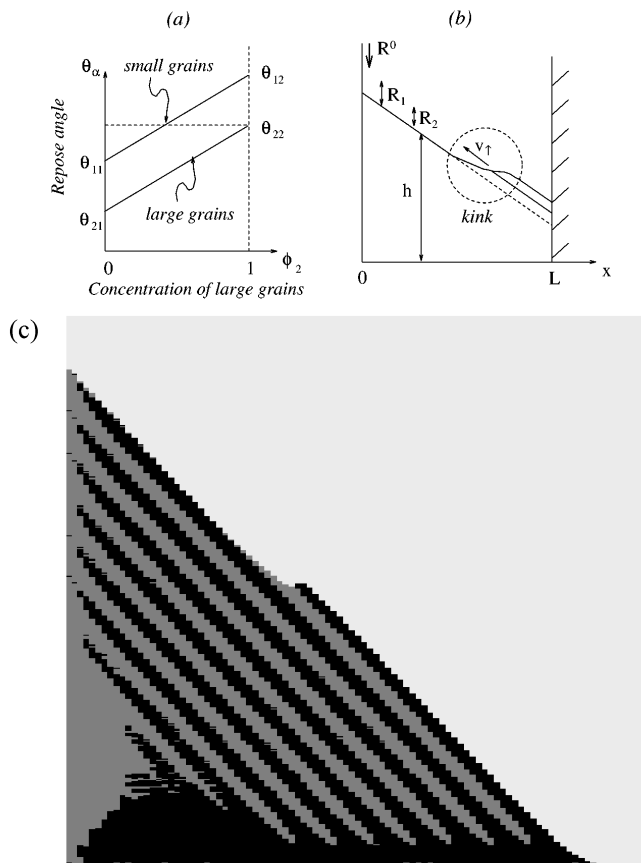
FIG. 2. (a) Dependence of the repose angle for the two types of rolling grains on the concentration of the surface of large grains \phi_2 . An essential ingredient to obtain stratification is that \theta_{22} > \theta_{11} . For the numerical integration, we use the linear interpolation between \phi_2 = 0 and \phi_2 = 1 as plotted here. (b) Picture with the different quantities appearing in the text. The dash-circled zone is the kink. (c) Resulting morphology of the numerical integration of the continuum equations. The parameters used are \tan \theta_{11} = 1 , \tan \theta_{22} = 1.1 , \tan \theta_{12} = 1.4 , \tan \theta_{21} = 0.7 , \gamma_1 = \gamma_2 = 0.8 , and v_1 = v_2 = 1 .
