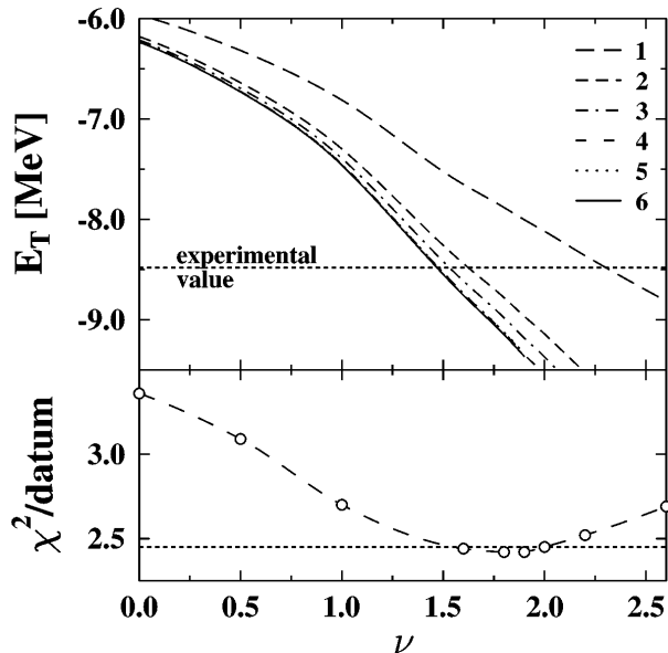
FIG. 1. Triton binding energy E_T for specific values of j_{\max} (upper panel) and \chi^2 for the fits to the two-body data (lower panel) versus the scalar meson off-shell parameter \nu defined in the text. The curves in both panels are smooth interpolations through the actual calculations. The lower panel also includes the line \chi^2 = 2.45 for reference.
