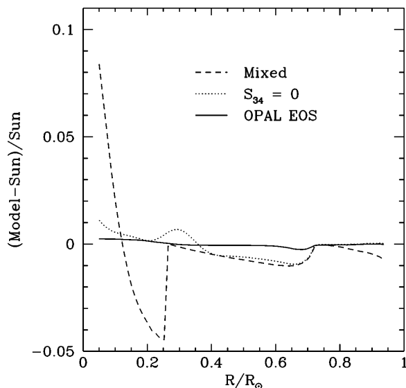
FIG. 2. Nonstandard solar models compared with helioseismology. This figure is similar to Fig. 1 except that the vertical scale is expanded. The dashed curve represents the sound speeds computed for the mixed solar model of Cumming and Haxton [11] with {}^3\text{He} mixing. The dotted line represents the sound speed for a solar model computed with the rate of the {}^3\text{He}(\alpha, \gamma){}^7\text{Be} reaction set equal to zero. For comparison, we also include the results for the new standard model labeled OPAL EOS in Fig. 1.
