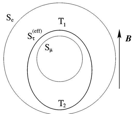
FIG. 1. If the resonant oscillation \nu_\tau \rightarrow \nu_e takes place between the electron neutrinosphere, S_e , and that of \nu_\mu, \nu_\tau, \bar{\nu}_\mu, \bar{\nu}_\tau , and \bar{\nu}_e, S_\mu , then the effective \tau neutrinosphere coincides with the surface of resonance, S_\tau^{(\text{eff})} . The latter is affected by the magnetic field. Therefore, the \tau neutrinos emitted in different directions come from the regions of different temperatures. The resulting anisotropy in the momentum of the outgoing neutrinos can be the origin of the pulsar kick velocity, whose magnitude depends on the magnetic field.
