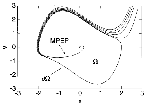
FIG. 1. The unstable limit cycle \partial\Omega of the van der Pol model, and the MPEP, which emerges from the attractor (0, 0) and spirals into it. The trajectories exiting from \Omega are optimal trajectories that are small perturbations of the MPEP.
