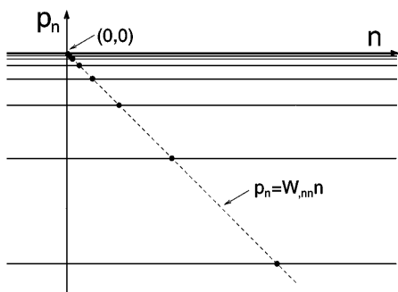
FIG. 2. A Poincaré section. This sketch shows the points (n, p_n) generated by the optimal trajectories passing by some specified point on \partial\Omega . The dots are generated by the MPEP, spiralling into \partial\Omega . Cf. Figs. 1–3 of Graham and Tél [10].
