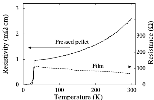
FIG. 1. Resistivity and resistance of the thin film and pressed pellet samples used in the optical and tunneling measurements, respectively.
