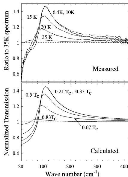
FIG. 2. (top) Far infrared transmission of the sample at temperatures below the superconducting transition. The curves are normalized to the transmission at T = 35 K in order to eliminate the features due to the silicon substrate. (bottom) Calculated transmission curves, based on dirty limit BCS results.
