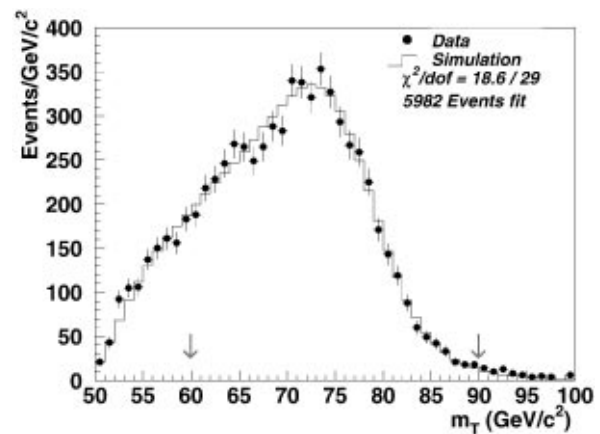
FIG. 3. Best fit to the transverse mass distribution. The arrows indicate the fitting range from which the W mass is extracted.
