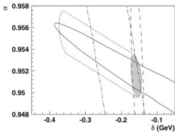
FIG. 1. Constraints on slope \alpha and intercept \delta from observed J/\psi \rightarrow e^+e^- (dash-dotted line), \pi^0 \rightarrow \gamma\gamma (dashed line), and Z \rightarrow e^+e^- decays (solid line). The shaded inner contour shows the combined result. The dotted line indicates the allowed area when nonlinear terms, as constrained by test beam measurements, are included.
