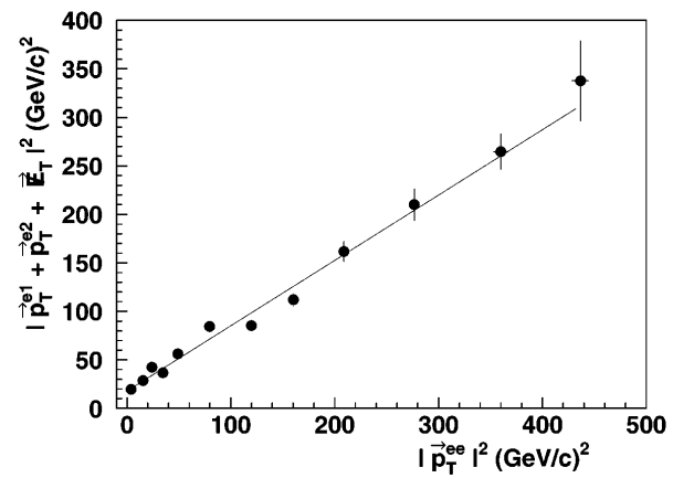
FIG. 2. Distribution of |\vec{p}_T^{e_1} + \vec{p}_T^{e_2} + \vec{E}_T|^2 versus |\vec{p}_T^{ee}|^2 for Z events
