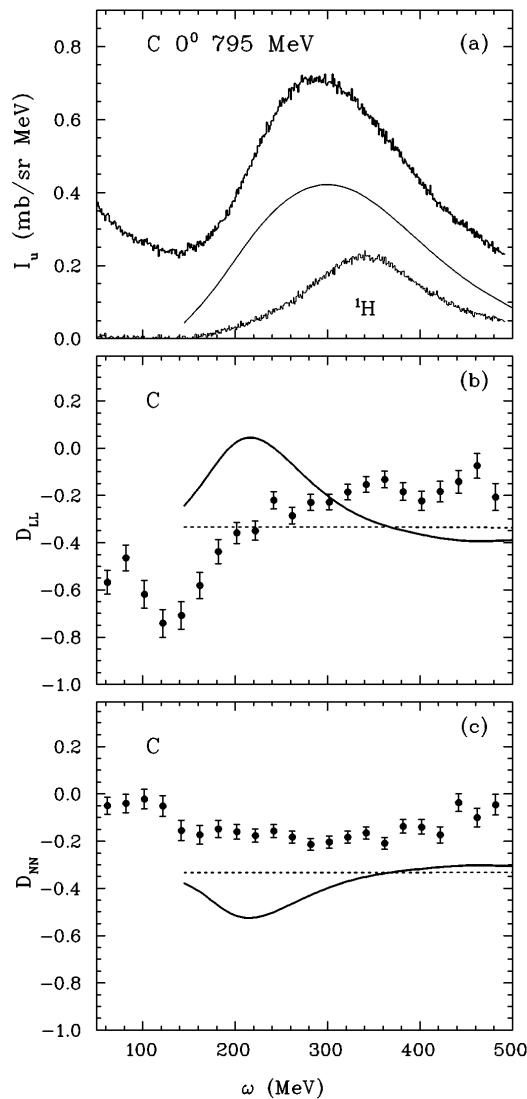
FIG. 1. In (a) the double differential cross sections for ^{12}\text{C}(p,n) (dark histogram) and ^1\text{H}(p,n) (light histogram) are shown. Below this appears the values for (b) D_{LL} and (c) D_{NN} for ^{12}\text{C}(\vec{p},\vec{n}) . The dark curves presented in these figures correspond to the result for the full (correlated) DWIA calculation that includes the residual interaction described in the text, while the dotted line in (b) and (c) represents the result from the same calculation with the residual interaction set to zero (uncorrelated).
