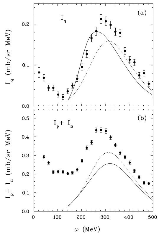
FIG. 2. The (a) spin-longitudinal and (b) spin-transverse partial cross sections for carbon are compared to the results of the DWIA calculations with (solid line) and without (dotted line) correlations.
