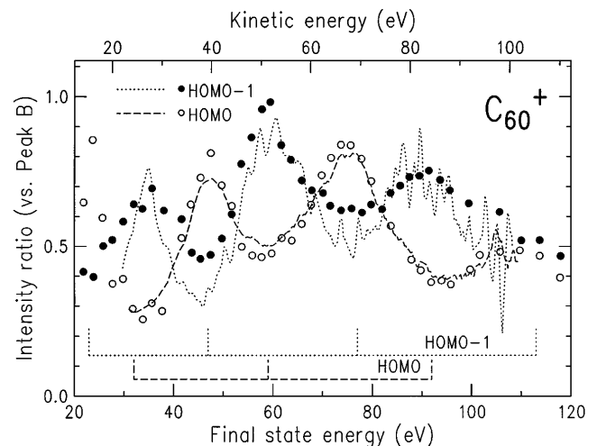
FIG. 1. Photoemission intensity variations as a function of final state energy ( E_f = E + IP_{\text{HOMO}} ) with respect to the HOMO level. The intensities from solid C_{60} from Ref. [3] (open and filled circles) are normalized to that of peak B (peak 4) which originates from a mixture of odd and even states [8]. The data from Ref. [4] (dashed and dotted line) have been normalized to the relative intensities of Ref. [6] before the ratio with respect to peak B was taken. The bar diagram indicates the minima positions in the partial cross sections (model A).
