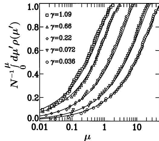
FIG. 2. Comparison between theory and simulation of the cumulative density of the variables \mu_n (related to the reflection eigenvalues by R_n = 1 + \mu_n^{-1} ). Curves are computed from the density (11) of the Laguerre ensemble; data points are from the simulation ( L = 500d = 19.2l, W = 151d, N = 63 ), for a single realization of the disorder.
