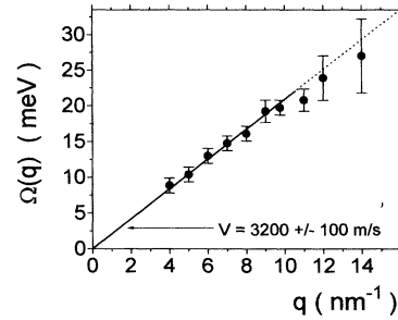
FIG. 3. Dispersion relation in water as obtained from the fit. The solid line indicates the best linear fit up to 10 \text{ nm}^{-1} , and the slope corresponds to the indicated speed of sound.
