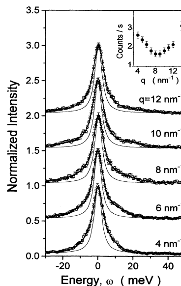
FIG. 1. Inelastic x-ray scattering spectra of \text{H}_2\text{O} at 294 K, taken at the indicated q values. The experimental data are normalized to the intensity of the central peak maximum, reported in the inset in counts/s. The data ( \circ ), shown with the error bars, are superimposed to the fit (solid line) as explained in the text. The line under the central peaks is the resolution function, shown to emphasize the q -dependent intensity on the sides of the central peak.
