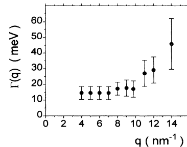
FIG. 4. Damping parameters \Gamma(q) as obtained from the fit.
