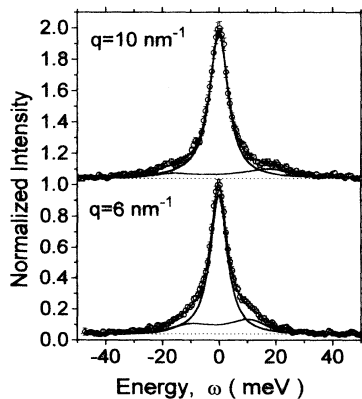
FIG. 2. Examples of fits to the data. The experimental data ( \circ ) are superimposed to the fit (solid line). The contribution of the central peak and the side peaks, due to the two terms in Eq. (1), are individually shown.
