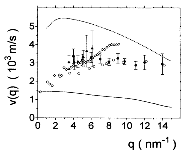
FIG. 5. Wave-vector dependence of different experimental and theoretical velocities of sound in water. \bullet , this work on \text{H}_2\text{O} ; \blacktriangle , neutron data on \text{D}_2\text{O} [3]; \circ , MD data on \text{D}_2\text{O} [10]; \diamond , MD data on \text{H}_2\text{O} [11]; solid (dashed) line, zero (infinite) frequency limit in \text{H}_2\text{O} [9].
