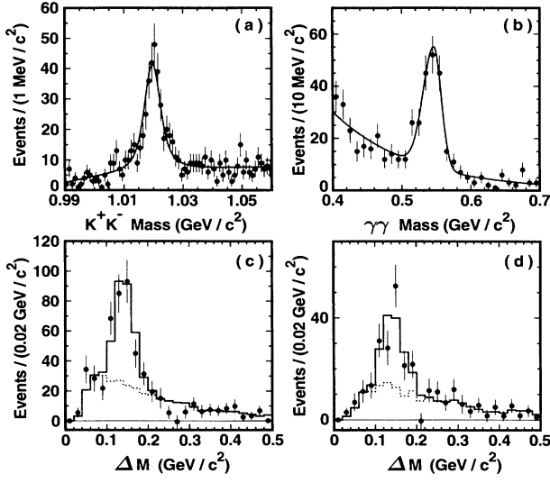
FIG. 2. The (a) K^+K^- and (b) \gamma\gamma invariant mass spectra for D_s^+ \rightarrow \phi \ell^+ \nu and D_s^+ \rightarrow \eta \ell^+ \nu candidates in the D_s^{*+} tag analysis: Note that a candidate photon from the D_s^{*+} is required. The solid curve is a fit to each spectrum. The spectra of the pseudomass difference \Delta M for (c) D_s^+ \rightarrow \phi \ell^+ \nu and (d) D_s^+ \rightarrow \eta \ell^+ \nu candidates: The points with error bars represent the number of candidates in each \Delta M bin. The solid histogram shows the simulated signal plus the predicted background, and the dotted histogram shows the predicted background. We removed the cut on \Delta M discussed in the text for (c) and (d).
