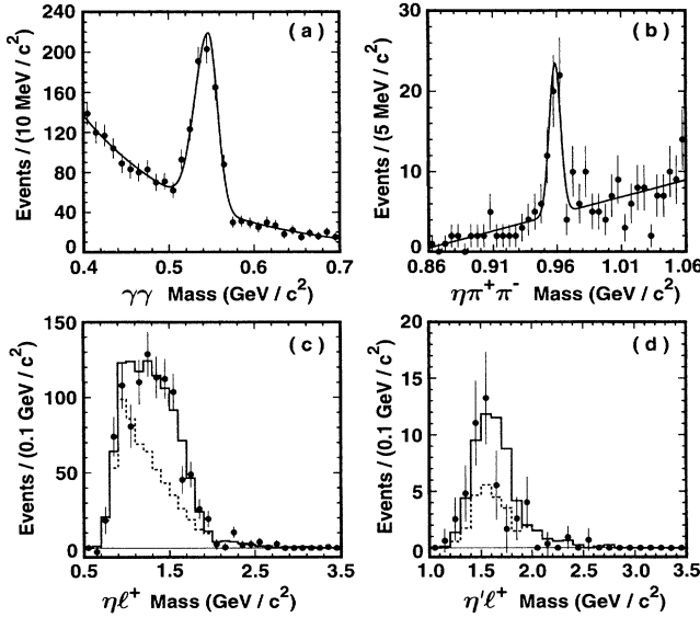
FIG. 1. The (a) \gamma\gamma and (b) \eta\pi^+\pi^- invariant mass spectra for D_s^+ \rightarrow \eta\ell^+\nu and D_s^+ \rightarrow \eta'\ell^+\nu candidates in the D_s^{*+} nontag analysis: The solid curve is a fit to each spectrum. (c) \eta\ell^+ and (d) \eta'\ell^+ are invariant mass spectra for the candidates: The points with error bars represent the number of candidates in each mass bin. The solid histogram shows the simulated signal plus the predicted background, and the dotted histogram shows the predicted background. We removed the cut on \eta\ell^+ and \eta'\ell^+ invariant masses discussed in the text for (c) and (d).
