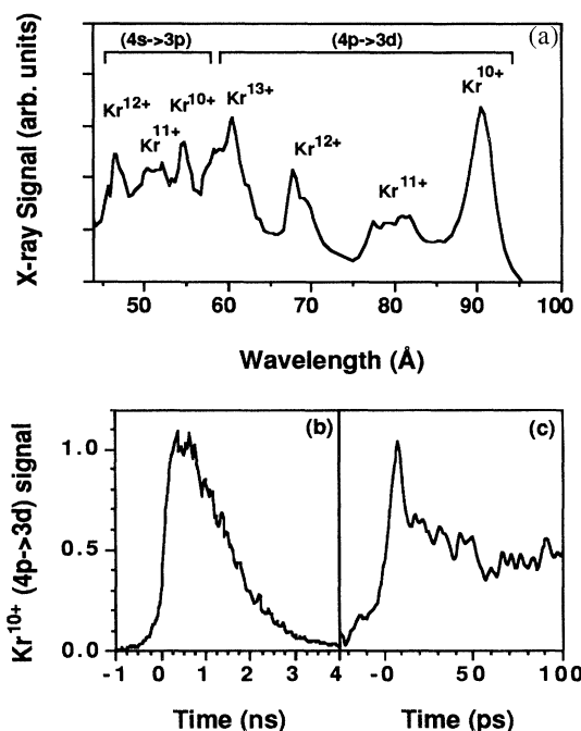
FIG. 3. (a) Time integrated spectrum produced in Kr (500 psi gas jet backing pressure) with an intensity of 1.5 \times 10^{16} W/cm ^2 . (b),(c) Measured time history of the Kr^{10+} 4p-3d line.
