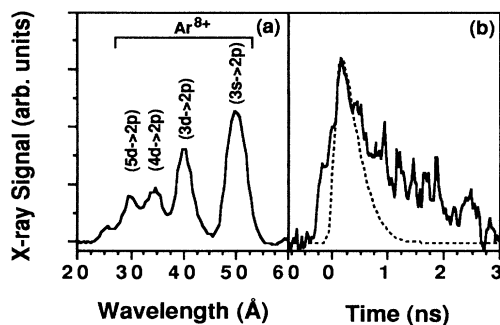
FIG. 4. (a) Time integrated spectrum produced in Ar (500 psi gas jet backing pressure) with an intensity of 8 \times 10^{15} W/cm 2 . (b) Measured (solid) and calculated (dashed) time history of the Ar 8+ 49 Å line.
