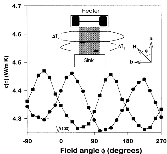
FIG. 1. Nominal thermal conductivities \kappa_1 (circles) and \kappa_2 (squares), determined from \Delta T_1 and \Delta T_2 , respectively, vs the field angle \phi . The lengths used are the vertical separations of the junctions sketched in the inset. The measurements are performed at T = 10 K and \mu_0 H = 1.5 T.
