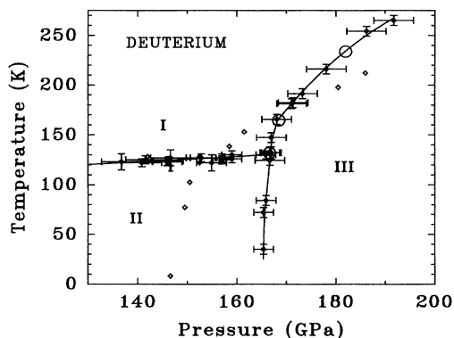
FIG. 1. Megabar phase diagram of deuterium. The small circles with error bars are from reversed isobaric temperature cyclings of this study. The larger open circles identify invariant points in the system. The diamonds are the results reported by Cui et al. [7].
