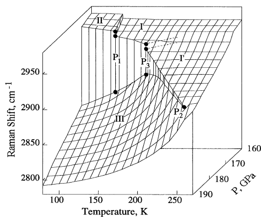
FIG. 5. Generalized P - T - \nu phase diagram for deuterium. p_1 , p_2 , and p_3 refer to the proposed invariant points.
