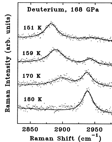
FIG. 2. Representative Raman spectra of the vibrons as a function of temperature at 168 GPa. The solid lines are fits to the data [28].
