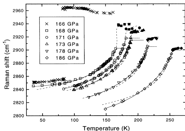
FIG. 4. Temperature dependence of the vibron frequencies for the I(II)-III transition at different pressures. Solid lines show T dependence of the order parameter for classical orientational ordering (Ref. [30]), defined as Q + 1/2 = 3 \int_0^1 x^2 \exp[x^2 U(Q + \gamma)/T] dx / \int_0^1 \exp[x^2 U(Q + \gamma)/T] dx . The dimensionless effective field \gamma changes from 0.008 (168 GPa) to 0.020 (188 GPa). Dashed lines show the phenomenological fit.
