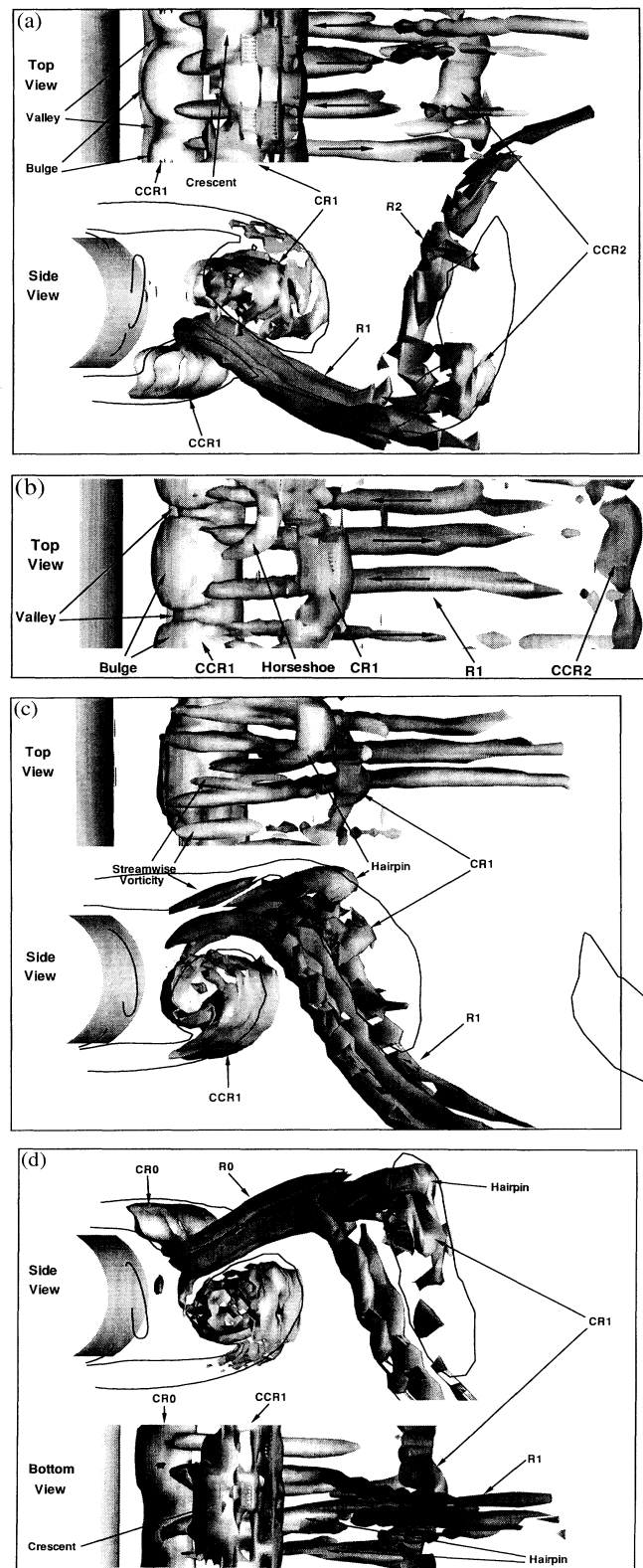
FIG. 1. Sequence of four plots showing vortical structures in the near wake visualized by |\lambda_i| = 1.1 over a time interval corresponding to about half of the shedding cycle.
