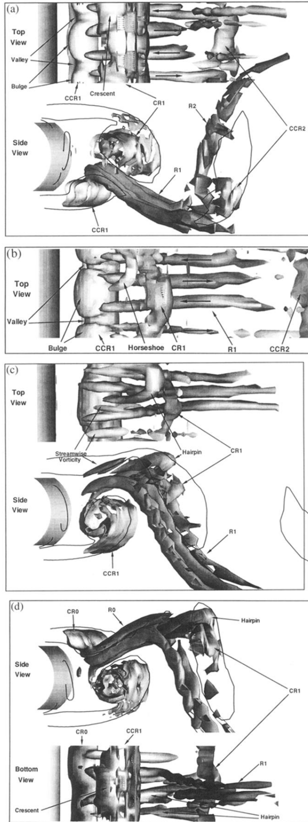
FIG. 1. Sequence of four plots showing vortical structures in the near wake visualized by |\lambda_i| = 1.1 over a time interval corresponding to about half of the shedding cycle.
