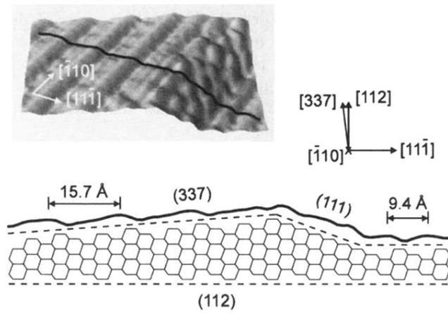
FIG. 3. Quantitative analysis of the nanofacet structure on Si(112). An image approximately 100 \text{ \AA} \times 40 \text{ \AA} ( \approx 10 \text{ \AA} height range) is shown along with a profile of the topography. The profile is also displayed over a cross section of the Si crystal structure, showing that the sawtooth is composed of short (111) and (337) facets.
