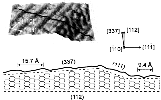
FIG. 3. Quantitative analysis of the nanofacet structure on Si(112). An image approximately 100 Å × 40 Å ( \approx 10 Å height range) is shown along with a profile of the topography. The profile is also displayed over a cross section of the Si crystal structure, showing that the sawtooth is composed of short (111) and (337) facets.
