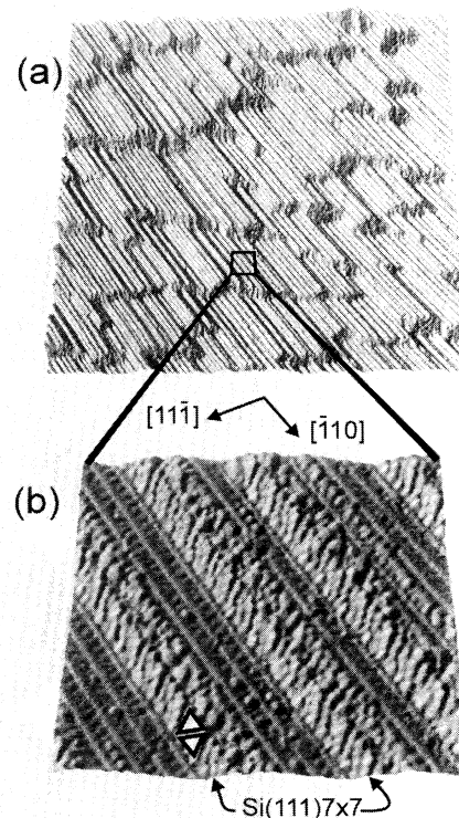
FIG. 4. Images of Si(335) revealing a nanofacet structure very similar to Si(112). (a) 5000 \text{ \AA} \times 5000 \text{ \AA} image ( 46 \text{ \AA} height range). The step bunches running approximately along [11\bar{1}] arise from a slight miscut of the wafer. (b) 300 \text{ \AA} \times 300 \text{ \AA} image ( 12 \text{ \AA} height range) showing the (337) and (111) nanofacets. One 7 \times 7 unit cell is highlighted.
