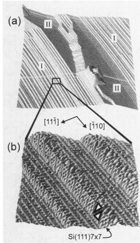
FIG. 2. Rendered STM topographs of Si(112). (a) 5000 \text{ \AA} \times 5000 \text{ \AA} image ( 340 \text{ \AA} height range) showing regions of quasiperiodic nanofacets (I) which are believed to be the equilibrium surface structure, and two large terraces (II) pinned by trace contaminants. (b) 320 \text{ \AA} \times 270 \text{ \AA} image ( 12 \text{ \AA} height range) of the nanofacets (filled states) showing a sawtoothlike structure. One 7 \times 7 unit cell on the (111) side of a sawtooth is highlighted. Note that this image is of a different sample than (a); the box is shown to indicate relative scale.
