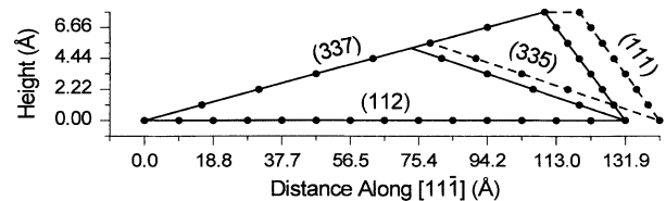
FIG. 5. Illustration of nanofacets on Si(112) and Si(335) which are composed of only a (337) terrace and a (111) terrace one 7 \times 7 unit cell wide (solid lines). Unit cell increments for the bulk-terminated surfaces are indicated by the filled circles. On the (335) surface the ideal facet structure is not coincident with the crystal structure. The dashed lines indicate a likely configuration for a coincident nanofacet on Si(335), composed of a (111) terrace one 7 \times 7 unit cell wide, two unit cells of (337), and a single unit of (112) on top of the sawtooth.
