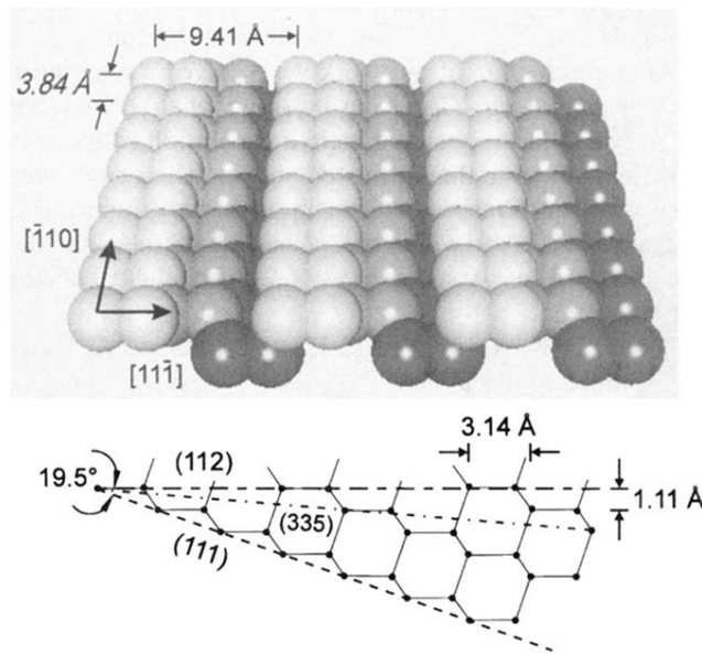
FIG. 1. A model of the bulk-terminated Si(112) surface. The bulk-terminated surface, which can be thought of as Si(111) tilted 19.5^\circ towards [\bar{1}\bar{1}2] , would consist of 8.87 \text{ \AA} wide (111) terraces separated by 3.14 \text{ \AA} high (001)-oriented steps. In the (112) plane the unit cell is 3.84 \text{ \AA} \times 9.41 \text{ \AA} . The -\cdot-\cdot- line indicates the (335) plane.
