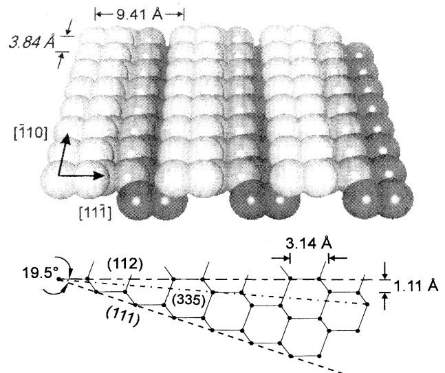
FIG. 1. A model of the bulk-terminated Si(112) surface. The bulk-terminated surface, which can be thought of as Si(111) tilted 19.5^\circ towards [\bar{1}\bar{1}2] , would consist of 8.87 \text{ Å} wide (111) terraces separated by 3.14 \text{ Å} high (001)-oriented steps. In the (112) plane the unit cell is 3.84 \text{ Å} \times 9.41 \text{ Å} . The — — — line indicates the (335) plane.
