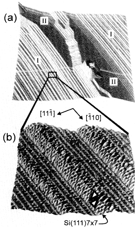
FIG. 2. Rendered STM topographs of Si(112). (a) 5000 Å × 5000 Å image (340 Å height range) showing regions of quasiperiodic nanofacets (I) which are believed to be the equilibrium surface structure, and two large terraces (II) pinned by trace contaminants. (b) 320 Å × 270 Å image (12 Å height range) of the nanofacets (filled states) showing a sawtoothlike structure. One 7 × 7 unit cell on the (111) side of a sawtooth is highlighted. Note that this image is of a different sample than (a); the box is shown to indicate relative scale.
