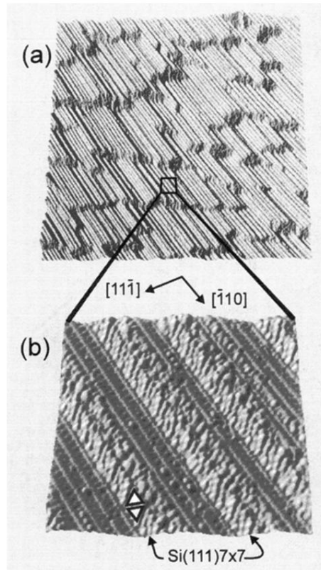
FIG. 4. Images of Si(335) revealing a nanofacet structure very similar to Si(112). (a) 5000 \text{ \AA} \times 5000 \text{ \AA} image ( 46 \text{ \AA} height range). The step bunches running approximately along [11\bar{1}] arise from a slight miscut of the wafer. (b) 300 \text{ \AA} \times 300 \text{ \AA} image ( 12 \text{ \AA} height range) showing the (337) and (111) nanofacets. One 7 \times 7 unit cell is highlighted.
