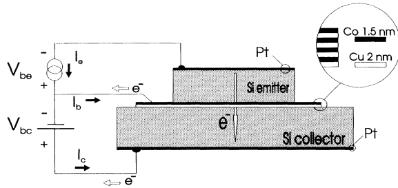
FIG. 1. Schematic cross section of the spin-valve transistor. A (Cu 2 nm/Co 1.5 nm) 4 multilayer base is rf sputtered onto the Si(100) collector substrate. The emitter has been direct-bonded to the base multilayer. Bias in the common base configuration and electron transport are shown for clarity. The base area is 2.7 \times 2.7 \text{ nm}^2 ; the emitter area is 1.6 \times 1.6 \text{ nm}^2 .
