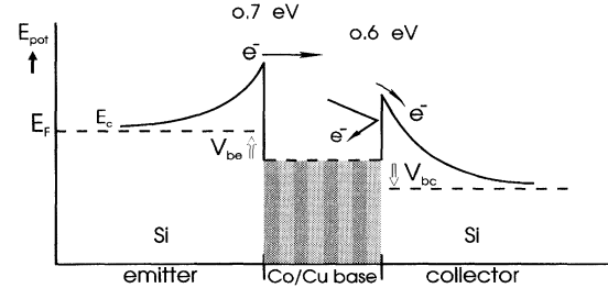
FIG. 2. Schematic energy band diagram of the spin-valve transistor under forward bias. The emitter Schottky barrier is slightly larger than the collector Schottky barrier, reducing quantum mechanical reflections. The collected electron current is exponentially dependent on the (inverse of the) MFP of the injected electrons in the Co/Cu multilayer base.
