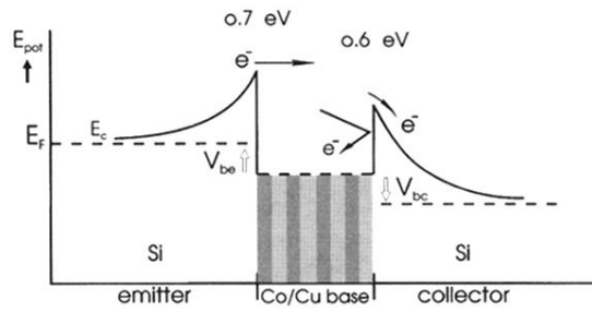
FIG. 2. Schematic energy band diagram of the spin-valve transistor under forward bias. The emitter Schottky barrier is slightly larger than the collector Schottky barrier, reducing quantum mechanical reflections. The collected electron current is exponentially dependent on the (inverse of the) MFP of the injected electrons in the Co/Cu multilayer base.
