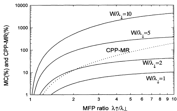
FIG. 3. Transmission characteristics of the spin-dependent transport. The relative change in magnetocurrent MC (%) and the relative change in perpendicular hot-electron spin valve effect in the base CPP-MR (%) are plotted versus the MFP ratio \lambda_{\uparrow}/\lambda_{\downarrow} .
