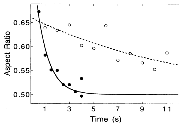
FIG. 1. Thermal relaxation of an atom cloud after one-dimensional heating. The figure shows the time variation of the aspect ratio of the cloud for two different initial densities (solid circles: 5 \times 10^{10} cm -3 ; open circles: 4 \times 10^9 cm -3 ). The lines represent simple exponential fits with time constants of 1.0 and 13 s, respectively.
