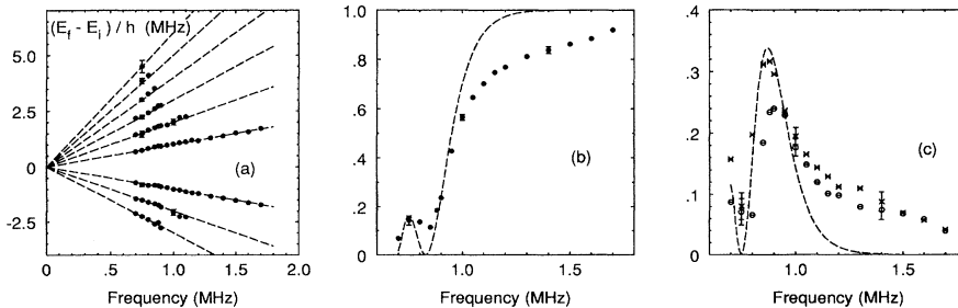
FIG. 4. (a) Energy transfers (deduced from arrival times at the probe) as a function of modulation frequency. The dotted lines show the theoretical prediction \Delta E_n/h = n\nu , with no fitted parameters. (b) Amplitude of the carrier and (c) amplitude of the sidebands n = -1 ( \times ) and n = 1 ( \circ ), as a function of modulation frequency; the dotted curves show an approximate theoretical prediction for reflection off an oscillating pure-exponential potential. The more efficient transfer seen experimentally above 1 MHz is related to the cutoff of the light shift potential at the dielectric surface. Experimental error bars, obtained by an analysis of the fitting procedure described in the text, have been plotted in (a)–(c) for all points at \nu = 0.75, 1, and 1.4 MHz.
