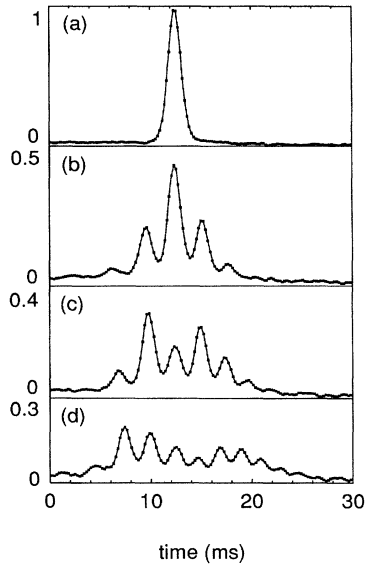
FIG. 3. Time-of-flight signals. (a) Nonmodulated potential; (b)–(d) modulated potential, with frequency \nu = 950 kHz (b), 880 kHz (c), and 800 kHz (d). The modulation depth is \epsilon = 0.82 . The width of the points indicates the time window for digitization and averaging of the continuous signal.
