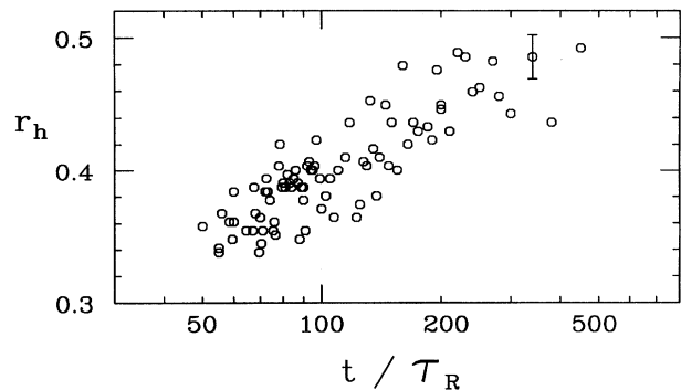
FIG. 5. Radial positions of symmetric two-hole configurations versus time.
