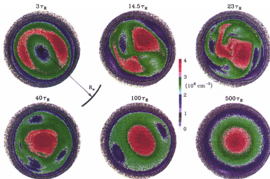
FIG. 2. False-color camera images of electron density (i.e., vorticity) showing the evolution of an initially hollow electron column.
