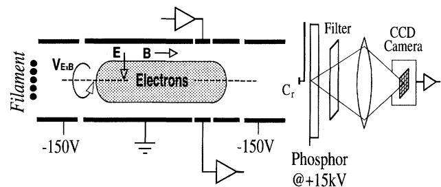
FIG. 1. The cylindrical experimental apparatus with phosphor screen/CCD camera diagnostic.
