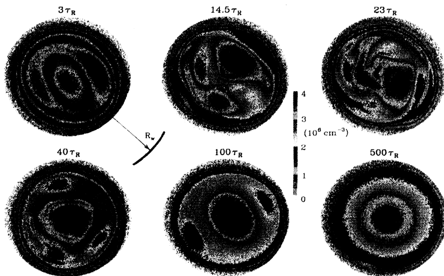
FIG. 2. False-color camera images of electron density (i.e., vorticity) showing the evolution of an initially hollow electron column.
