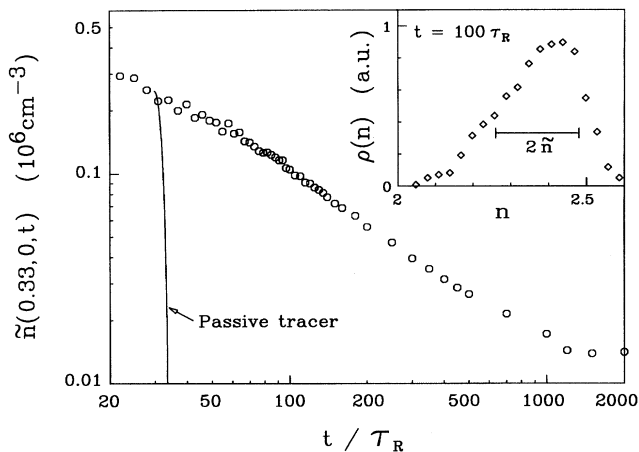
FIG. 6. Measured fluctuation level \tilde{n} vs time, and predicted passive tracer mixing. The inset shows the PDF \rho(n) .
