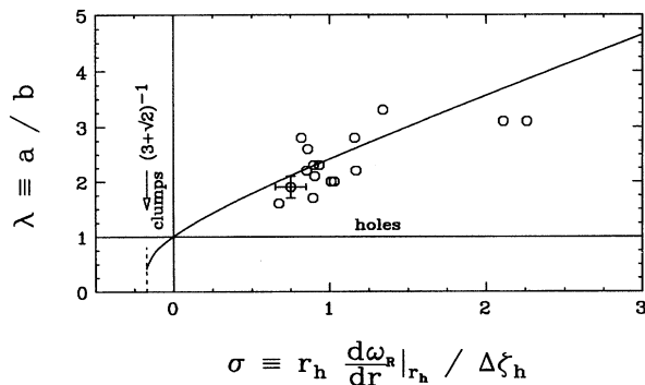
FIG. 4. Measured hole aspect ratio \lambda vs normalized background shear \sigma and Moore-Saffman model (curve).
