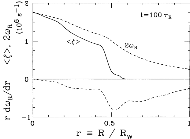
FIG. 3. Radial profiles of the \theta averaged vorticity \langle \zeta \rangle , rotation \omega_R , and shear r d\omega_R/dr .
