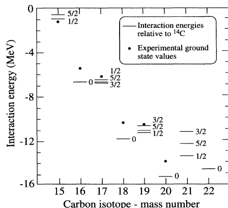
FIG. 2. Calculated interaction energies relative to ^{14}\text{C} (lines labeled by the J value) compared to the experimental ground state energies (filled circles).
