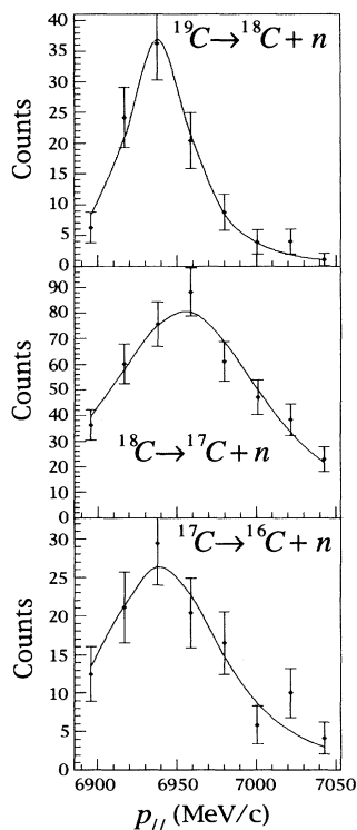
FIG. 1. Longitudinal momentum distributions of the recoiling fragment in the one-neutron breakup of ^{19}\text{C} , ^{18}\text{C} , and ^{17}\text{C} .
