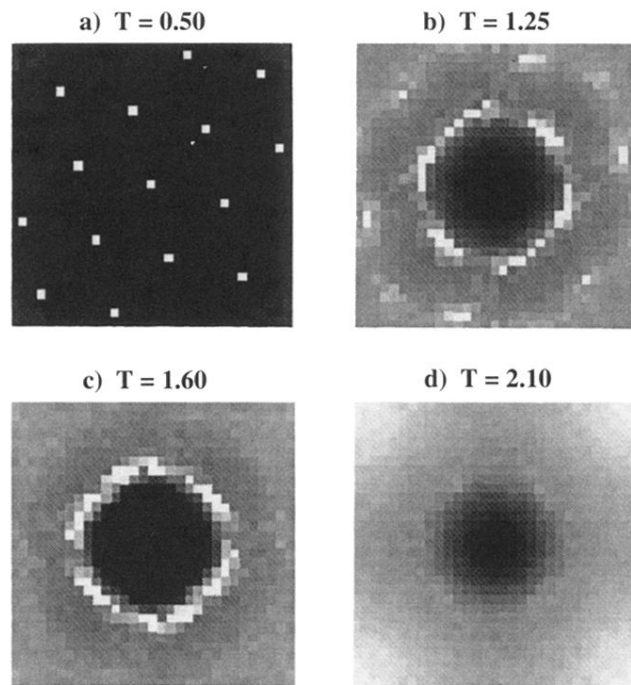
FIG. 3. Intensity plot of S(\mathbf{q}_\perp) for several T and L_\perp = L_z = 30 . (a) T = 0.50 < T_m shows a lattice of Bragg peaks; (b) T = 1.25 \approx T_m ; (c) T_m < T = 1.60 < T_c in the vortex line liquid; and (d) T = 2.10 > T_c .
