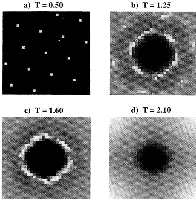
FIG. 3. Intensity plot of S(\mathbf{q}_\perp) for several T and L_\perp = L_z = 30 . (a) T = 0.50 < T_m shows a lattice of Bragg peaks; (b) T = 1.25 \approx T_m ; (c) T_m < T = 1.60 < T_c in the vortex line liquid; and (d) T = 2.10 > T_c .
