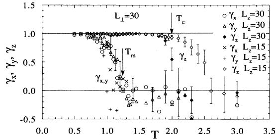
FIG. 2. \gamma_\mu vs T for L_\perp = 30 and L_z = 15, 30 . Sample error bars are shown. \gamma_{x,y} decreases at T_m \approx 1.2 ; \gamma_z decreases at T_c \approx 2.0 .
