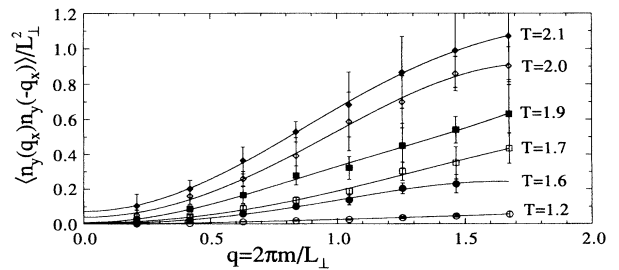
FIG. 1. \langle n_y(q_x)n_y(-q_x) \rangle / L_\perp^2 vs q_x = 2\pi m / L_\perp ( m integer) for various T and L_\perp = L_z = 30 . Solid lines are a fit by Eq. (5).
