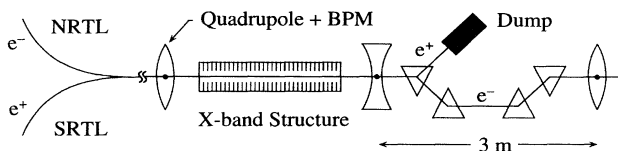
FIG. 1. Layout of ASSET in the SLC.
