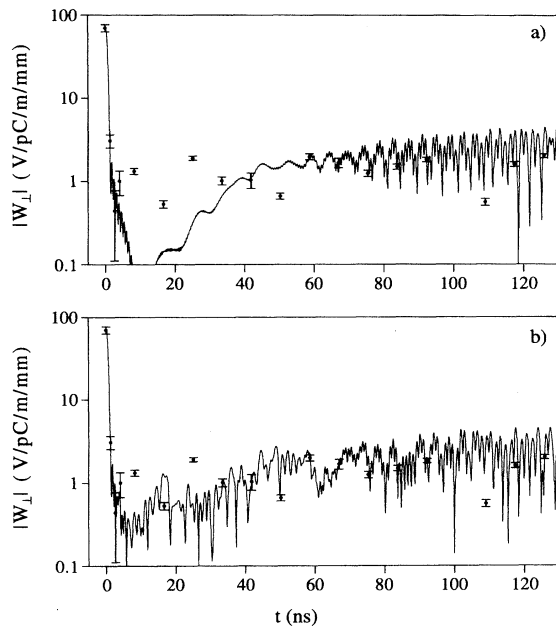
FIG. 3. Dipole wake-field amplitude measurements and prediction (a) without cell frequency errors and (b) with 1.5 \times 10^{-4} rms fractional frequency errors.
