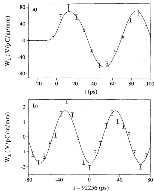
FIG. 2. Dipole wake field measured (a) near the bunch crossing and (b) at a bunch separation of about 92 ns. The solid lines are described in the text.
