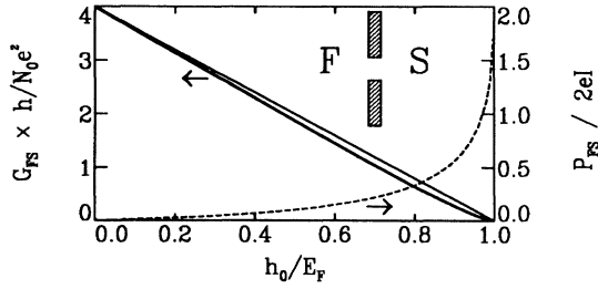
FIG. 1. The conductance G_{FS} (full curves) and the shot-noise power P_{FS} (dashed) of a ballistic point contact in a ferromagnet-superconductor junction (see inset), as a function of the exchange energy h_0 . The thick line represents the exact result (7) for G_{FS} , the thin line the estimation (2).
