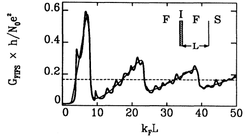
FIG. 2. The conductance G_{FIFS} of a clean FIFS junction containing a planar tunnel barrier (transparency \Gamma ) on the ferromagnetic side, as a function of the separation L from the interface (see inset). The thick solid line is computed from Eq. (9) for \Gamma = 0.1 , h_0 = 0.2E_F . For the thin line normal reflection at the FS interface is neglected ( r_{ee} = 0 ). The dashed line is the classical large- L limit.
