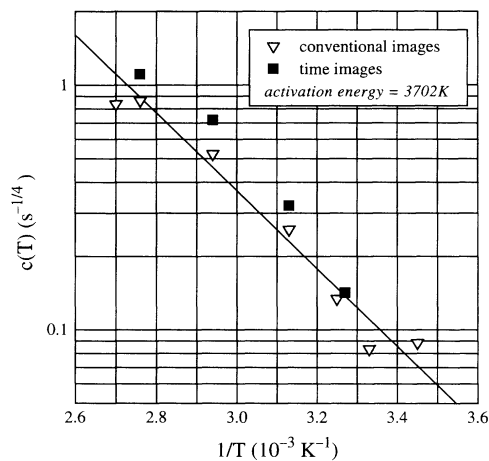
FIG. 3. Arrhenius plot of c(T) defined in Eq. (6). The triangles and squares refer to data obtained from conventional and time images, respectively.
