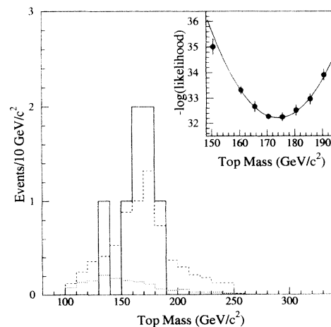
FIG. 2. Top mass distribution for the data (solid histogram), the W +jets background (dots), and the sum of background + Monte Carlo t\bar{t} for M_{\text{top}} = 175 GeV/ c^2 (dashed). The background distribution has been normalized to the 1.4 background events expected in the mass-fit sample. The inset shows the \ln(\text{likelihood}) fit used to determine the top mass.
