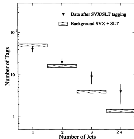
FIG. 1. The sum of SVX and SLT tags observed in the W +jets data (solid triangles). Events tagged by both algorithms are counted twice. The shaded area is the sum of the background estimates for SVX and SLT, with its uncertainty. The three-jet and four-or-more-jet bins are the t\bar{t} signal region.
