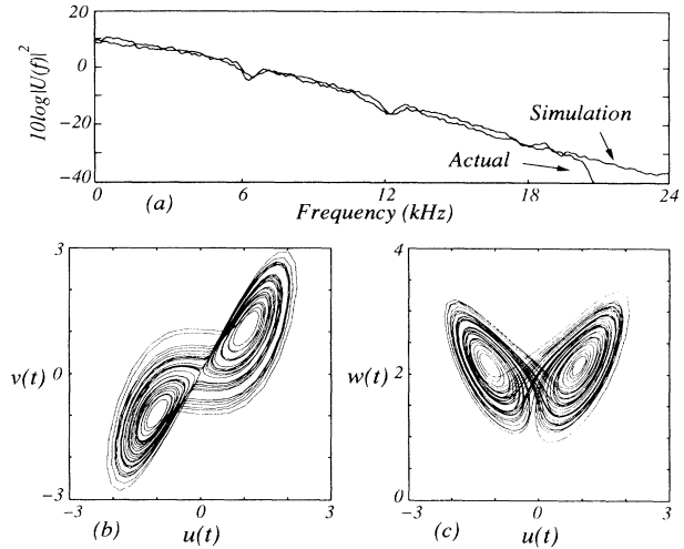
FIG. 2. Circuit data: (a) averaged power spectrum of u(t) ; (b) chaotic attractor projected onto the uv plane; (c) chaotic attractor projected onto the uw plane.
