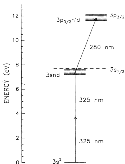
FIG. 1. The excitation path used in the experiment is shown. Two photons of doubled 650 nm light excited Mg to a 3snd\ ^1D_2 Rydberg wave packet state, where n is the central state of the wave packet. One photon of the doubled 560 nm light then excited the 3s core electron, producing 3p_{3/2}n'd autoionizing states, where n' is the central state of the final Rydberg wave packet.
