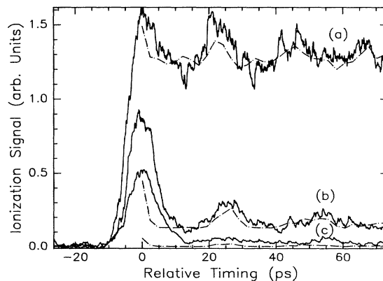
FIG. 3. Measured and calculated spectra are shown for several tunings of the core laser with the Rydberg laser tuned to n=54 . Near the ionic resonance, (a), a large baseline signal results from the resonant excitation of the core electron which is largely independent of the position of the Rydberg electron. Away from the ionic resonance (b) and (c), the shakeup excitation exhibits a strong dependence on the Rydberg electron position.
