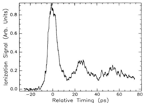
FIG. 2. A time resolved excitation spectrum is shown where the initial Rydberg state is centered around n=54 and the core laser is tuned approximately 15\text{ cm}^{-1} to the blue of the ionic resonance. The time axis represents the relative timing between the Rydberg and core laser. Peaks are seen in the excitation spectrum when the relative timing is equal to an integral number of classical orbital periods of the central Rydberg state of the wave packet. For n=54 the classical orbital period is 24 ps.
