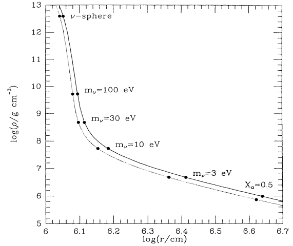
FIG. 1. Matter density profiles from numerical supernova models at late times. The solid line is for t_{\text{PB}} \approx 4 \text{ s} and the dotted line is for t_{\text{PB}} \approx 6 \text{ s} . Also shown are the position of the neutrinosphere and the positions of neutrino mass-level crossings for a 25 MeV neutrino for the cases where the heavier vacuum neutrino mass is m_\nu = 100, 30, 10 , and 3 \text{ eV} . The location where the alpha-particle mass fraction is 0.5 is shown.
