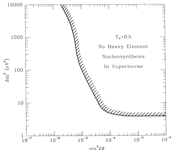
FIG. 2. The Y_e=0.5 line is shown on a plot of vacuum mass-square difference \delta m^2 versus \sin^2 2\theta . The region to the right of the Y_e=0.5 line is excluded if supernovae are to produce r -process heavy elements.
