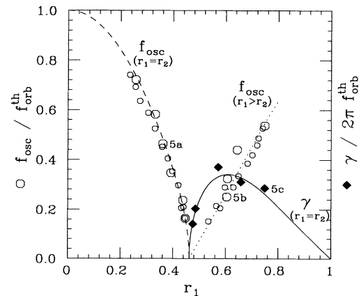
FIG. 4. Normalized measured oscillation frequencies f_{\text{osc}} ( \circ ) and exponential growth rates \gamma ( \diamond ). The curves show predictions from an analytic point vortex model, where the solid line indicates exponential growth and the dashed and dotted lines are oscillation frequencies. The motions corresponding to the three marked rates are shown in Figs. 5(a)-5(c).
