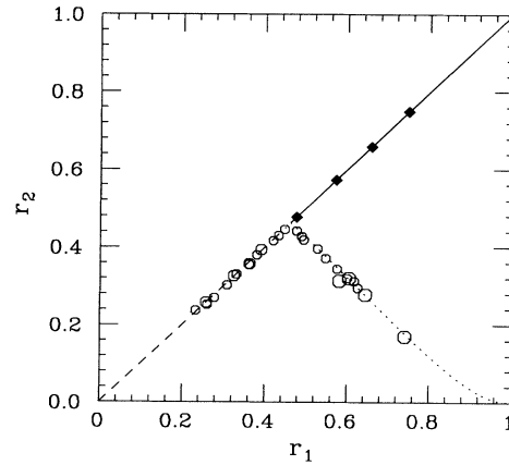
FIG. 3. Measured radial positions of stable ( \circ ) and unstable ( \diamond ) equilibrium points, where \theta_2 = \theta_1 + \pi for all points. The size of the symbol indicates the estimated uncertainty. The predictions of the point vortex model are also plotted for stable (dashes, dots) and unstable (solid line) points.
