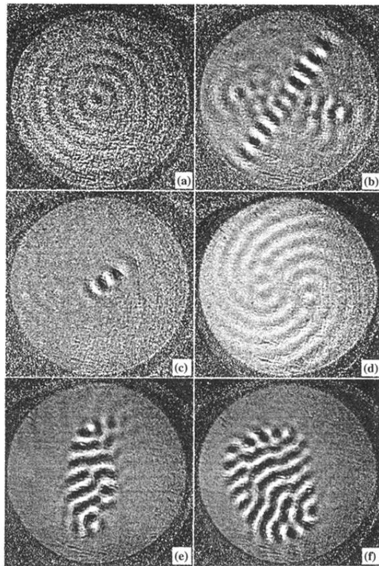
FIG. 4. Shadowgraph images showing the subsequent (rather atypical) evolution observed in the run shown in Figs. 1(b)–1(f). Image (a) was taken 370t_r after image (f) of Fig. 1, and is shown here with enhanced contrast. Subsequent images were taken at intervals of 70t_r .
