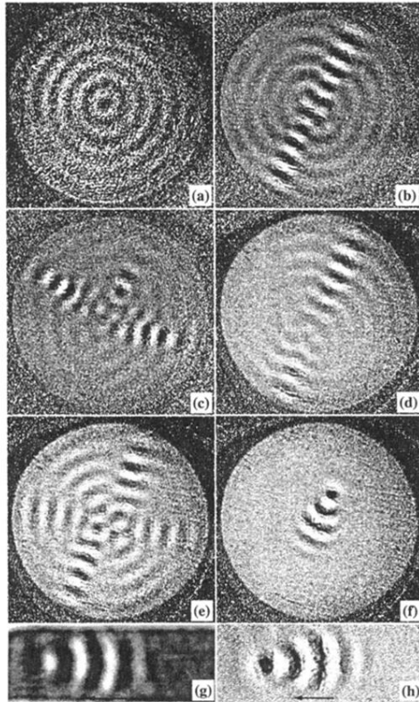
FIG. 1. Shadowgraph images showing the initial transient leading to convection in a water/ethanol mixture having a separation ratio \psi = -0.09 . Images (a)–(f) were obtained using a circular cell of radial aspect ratio 11.6, with \Delta T barely above \Delta T_c . (b)–(f) were taken at intervals of 100t_c (3 h), while image (a) is from a different run and shown with an enhanced contrast. In (g) and (h), a stable pulse (g) observed in a rectangular cell of width 4.87 and length 25.3 times its depth ( \psi = -0.09 ; see Ref. [2]) is compared to the 2D pulse (h) from image (f). The pulse from (f) was expanded and rotated. The arrows in images (g) and (h) indicate the direction of roll propagation.
