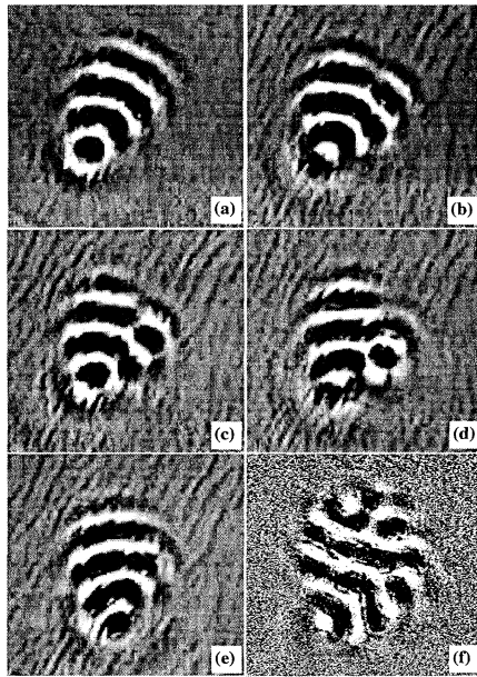
FIG. 2. Shadowgraph images showing the typical evolution of a localized pulse of convection which is expanding at \epsilon=0.0010 in a mixture with \psi=-0.10 . Image (a) shows the pulse shortly after its formation. Image (b), taken about 30t_c later, shows that the pulse has spread somewhat and is becoming unstable on its trailing edge, where the waves enter. Images (c) and (d) show the resulting defect traveling along the pulse, leaving it essentially unchanged, but reoriented [image (e)]. Images (b) through (e) were taken at intervals of about 3t_c . Image (f), which is from another run with \psi=-0.10 and \epsilon=-0.0031 , shows a typical disordered but still localized state which results (usually after many cycles of reorientation) when the pulse retains several of these defects.
