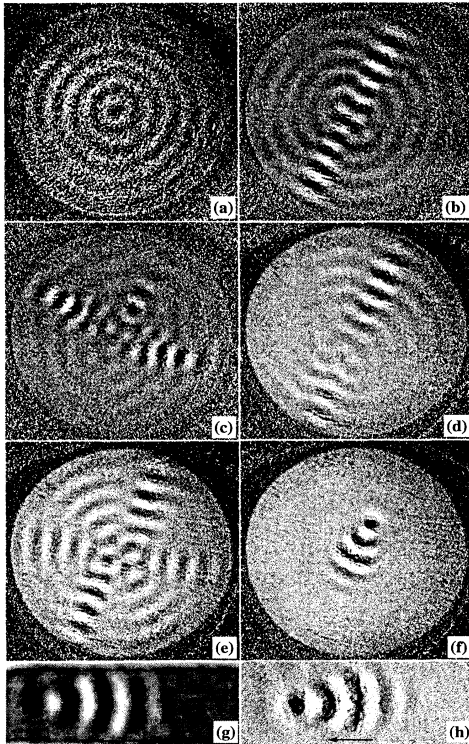
FIG. 1. Shadowgraph images showing the initial transient leading to convection in a water/ethanol mixture having a separation ratio \psi = -0.09 . Images (a)–(f) were obtained using a circular cell of radial aspect ratio 11.6, with \Delta T barely above \Delta T_c . (b)–(f) were taken at intervals of 100t_v (3 h), while image (a) is from a different run and shown with an enhanced contrast. In (g) and (h), a stable pulse (g) observed in a rectangular cell of width 4.87 and length 25.3 times its depth ( \psi = -0.09 ; see Ref. [2]) is compared to the 2D pulse (h) from image (f). The pulse from (f) was expanded and rotated. The arrows in images (g) and (h) indicate the direction of roll propagation.
