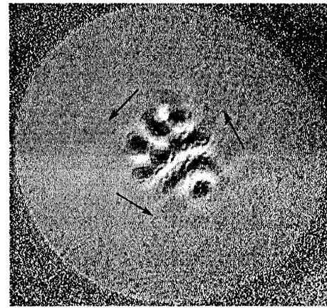
FIG. 3. Shadowgraph image of a localized state obtained at \psi=-0.14 by reducing the heat current to 0.977 of its critical value during the initial transient. After about 1700t_c (over 2 d) this state began to expand. Arrows indicate the direction of traveling-wave motion.
