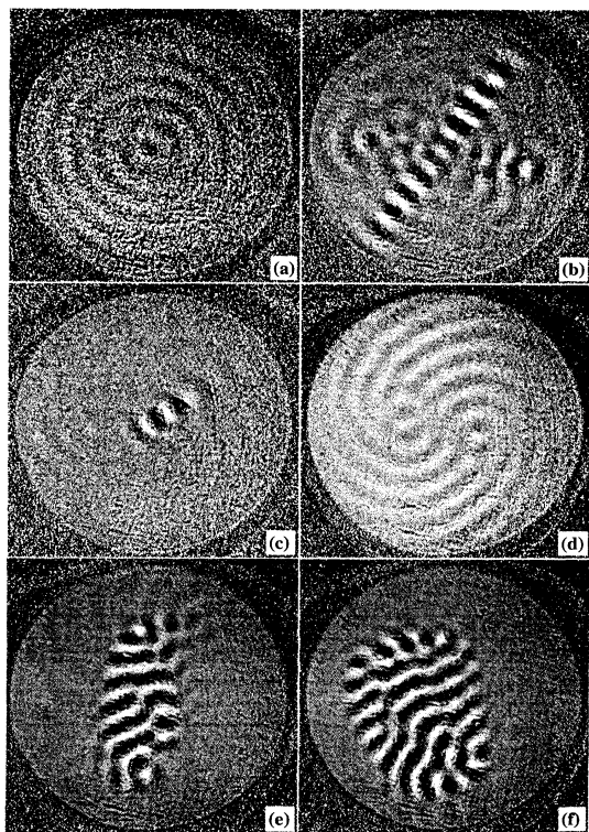
FIG. 4. Shadowgraph images showing the subsequent (rather atypical) evolution observed in the run shown in Figs. 1(b)–1(f). Image (a) was taken 370t_c after image (f) of Fig. 1, and is shown here with enhanced contrast. Subsequent images were taken at intervals of 70t_c .
