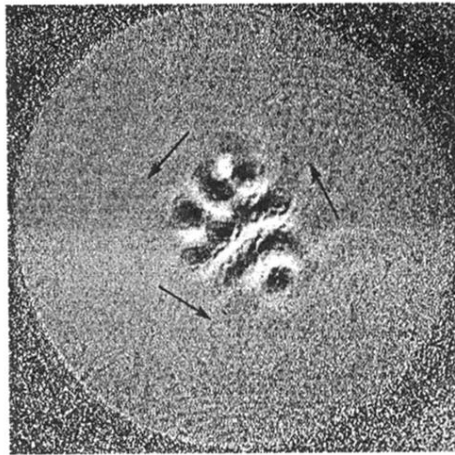
FIG. 3. Shadowgraph image of a localized state obtained at \psi = -0.14 by reducing the heat current to 0.977 of its critical value during the initial transient. After about 1700t_r (over 2 d) this state began to expand. Arrows indicate the direction of traveling-wave motion.
