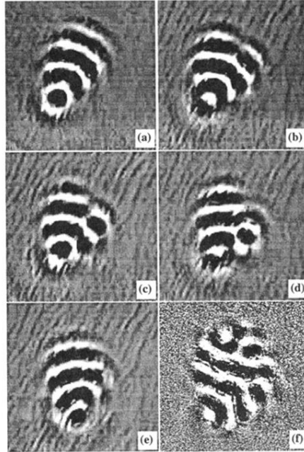
FIG. 2. Shadowgraph images showing the typical evolution of a localized pulse of convection which is expanding at \epsilon=0.0010 in a mixture with \psi=-0.10 . Image (a) shows the pulse shortly after its formation. Image (b), taken about 30t_e later, shows that the pulse has spread somewhat and is becoming unstable on its trailing edge, where the waves enter. Images (c) and (d) show the resulting defect traveling along the pulse, leaving it essentially unchanged, but reoriented [image (e)]. Images (b) through (e) were taken at intervals of about 3t_e . Image (f), which is from another run with \psi=-0.10 and \epsilon=-0.0031 , shows a typical disordered but still localized state which results (usually after many cycles of reorientation) when the pulse retains several of these defects.
