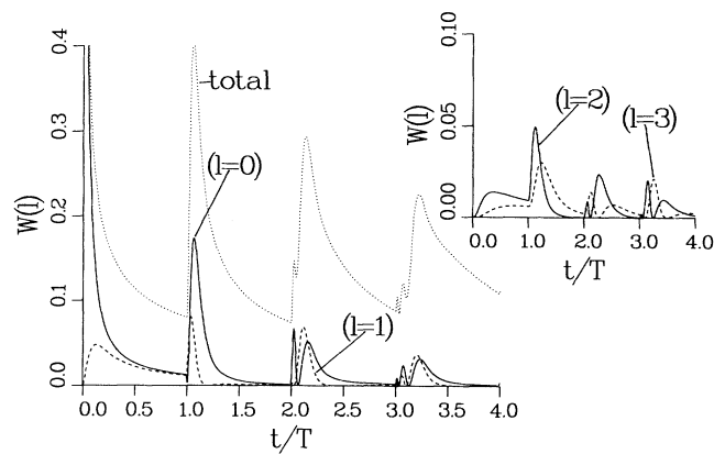
FIG. 2. W(l) = |a_g^{(l)}(t)|^2 as a function of the interaction time t = L/v_{in} in units of T for \delta\omega = 0 , \gamma T = 50.0 , and e^{2i\pi(\bar{\nu}+a)} = 1.0 . The total initial state probability (total) is also shown.
