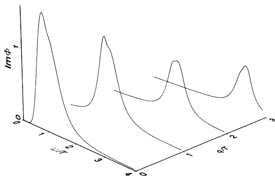
FIG. 2. The imaginary part of the universal susceptibility in the QC region, \Phi , as a function of x = \hbar c q/k_B T and y = \hbar \omega/k_B T for a nonrandom square lattice AFM which undergoes a T=0 transition from Néel-LRO to a QD phase. The results have been computed in a 1/N expansion to order 1/N and evaluated for N=3 . The two-loop diagrams were analytically continued to real frequencies and the integrals then evaluated numerically. The shoulder on the peaks is due to a threshold towards three-spin-wave decay.
