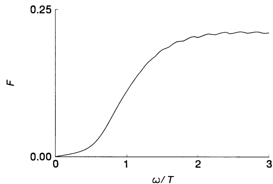
FIG. 3. The imaginary part of the universal local susceptibility, F , for the same model as in Fig. 2. We have F(y) = y^{-\mu} \int d\vec{x} \text{Im}\Phi(\vec{x}, y) . The oscillations at large y are due to a finite step size in the momentum integrations.
