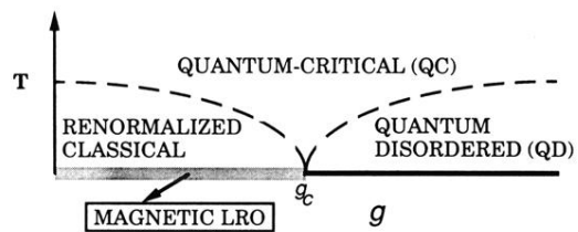
FIG. 1. Phase diagram of \mathcal{H} (after Ref. [4]). The magnetic LRO can be either spin-glass or Néel type, and is present only at T=0 . The boundaries of the QC region are T \sim |g - g_c|^{2\nu} . For nonrandom \mathcal{H} which have commensurate, collinear, Néel LRO for g < g_c , all of the QD region ( g > g_c ) has spin-Peierls order at T=0 —this order extends to part of the QD region at finite T .
