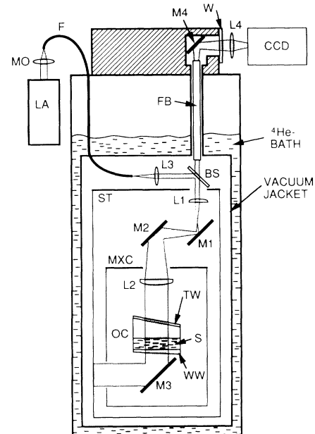
FIG. 1. Schematic illustration of the experimental setup (not to scale). Explanation of symbols: MO, microscope objective; M1, . . . , M4, aluminum coated mirrors; W, window. For other abbreviations, see text.
