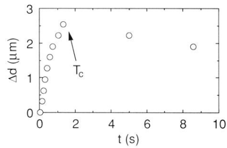
FIG. 4. Upper part: Illustration of the shrinking interference rings in the superfluid state due to the fountain effect. From left to right, the three pictures were taken at 20-ms intervals, and their contrast was increased by subtracting successive frames as in Fig. 2. Lower part: Increase of the sample thickness \Delta d as a function of time after illumination at the maximum attainable light power was started when T < T_c . Each datum corresponds to a change by one-half of the optical wavelength. The thickness of the ^3\text{He} layer at start was d = 0.5 mm.
