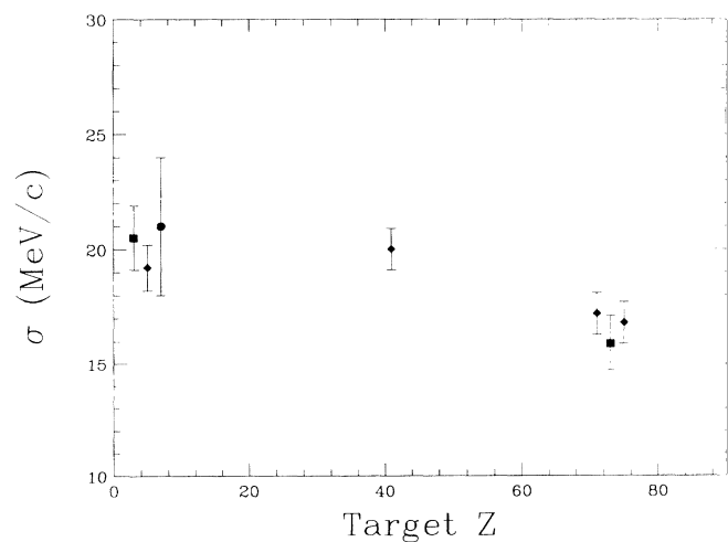
FIG. 2. Target Z dependence of the widths (Table I) of the momentum distributions for the medium (squares) and high (diamonds) acceptance mode measurements. The result of Kobayashi et al. [10] is indicated by the circle.
