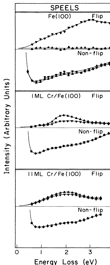
FIG. 4. Flip and nonflip partial scattering rates as a function of energy loss for several thicknesses of Cr on Fe. \blacktriangle and \blacktriangledown indicate incident electron spins up and down, respectively, relative to the Fe majority spin direction.
